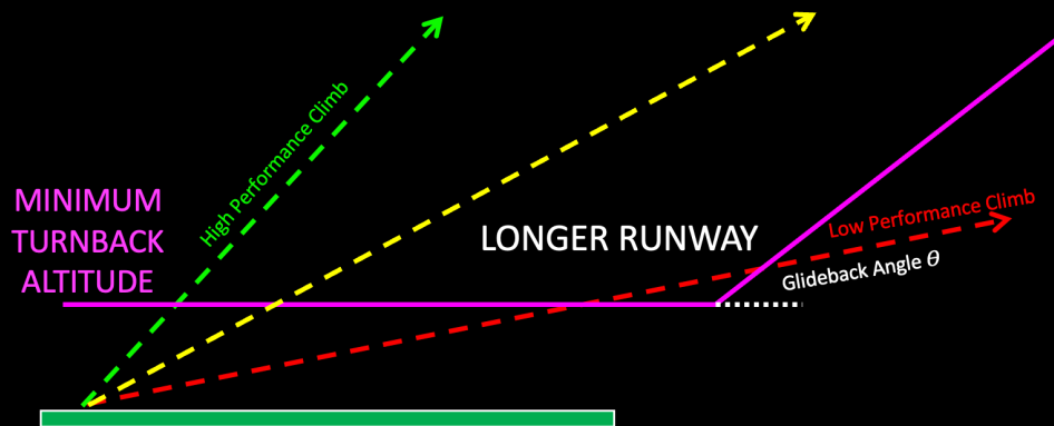
CLIMB PERFORMANCE, RUNWAY LENGTH, ALTITUDE LOST IN TURNBACK, AND GLIDEBACK DESCENT ANGLE DETERMINE TURNBACK POTENTIAL
