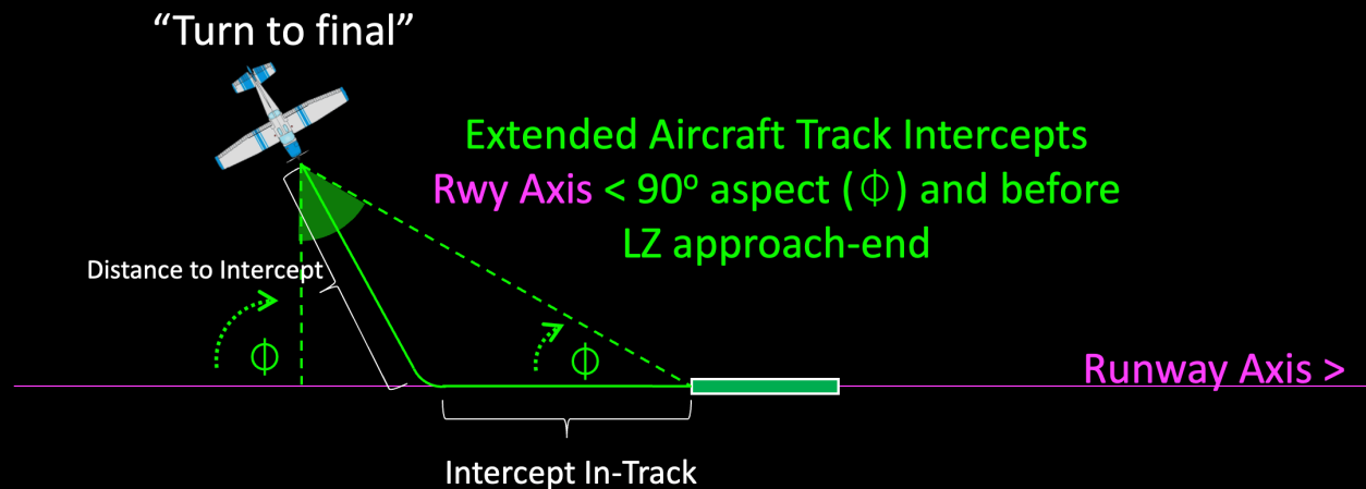
Figure 48 – Base Turn to Final
